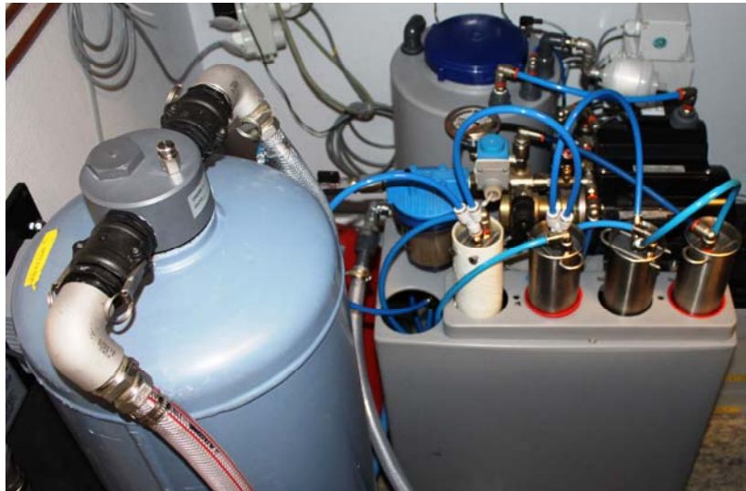
Fig. 2. The installed equipment used for cleaning printed circuit boards according to the Qlean-method at Flextronics in Karlskrona, Sweden.
